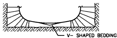
FIG. 5 Bedding and Corner Zone Treatment for Pipe Arch Structures
